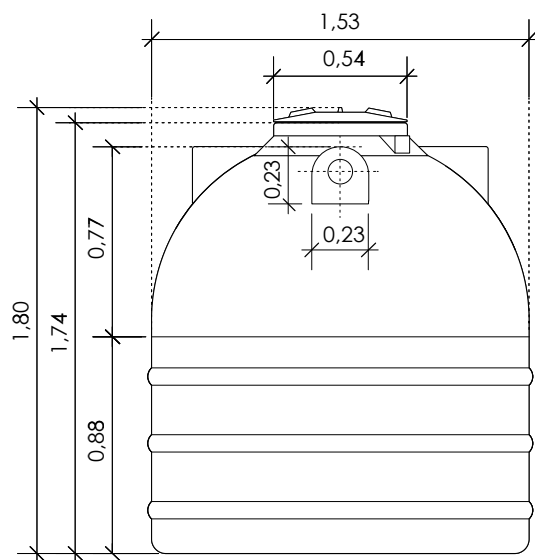
VISTA FRONTAL
