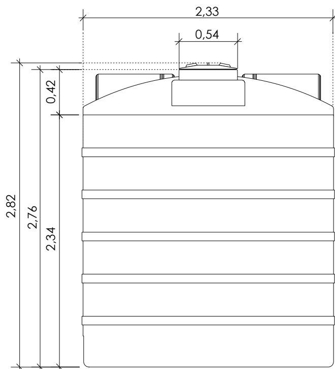
VISTA FRONTAL
